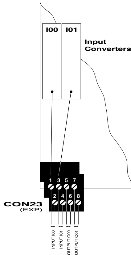
Figure 3-7—On-Board Digital I/O (Expandable Control Modules)
