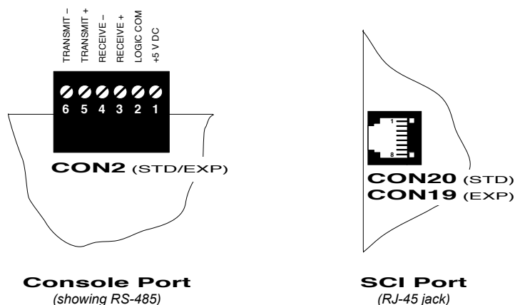
Figure 3-3—Asynchronous Serial Connections
