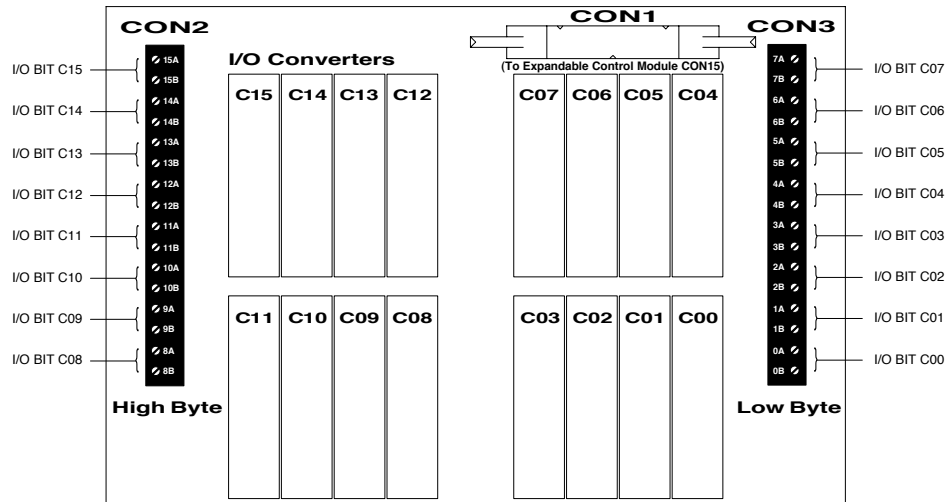
Figure 3-8—16-Bit Fanning Strip Expanded Digital I/O (320102)
