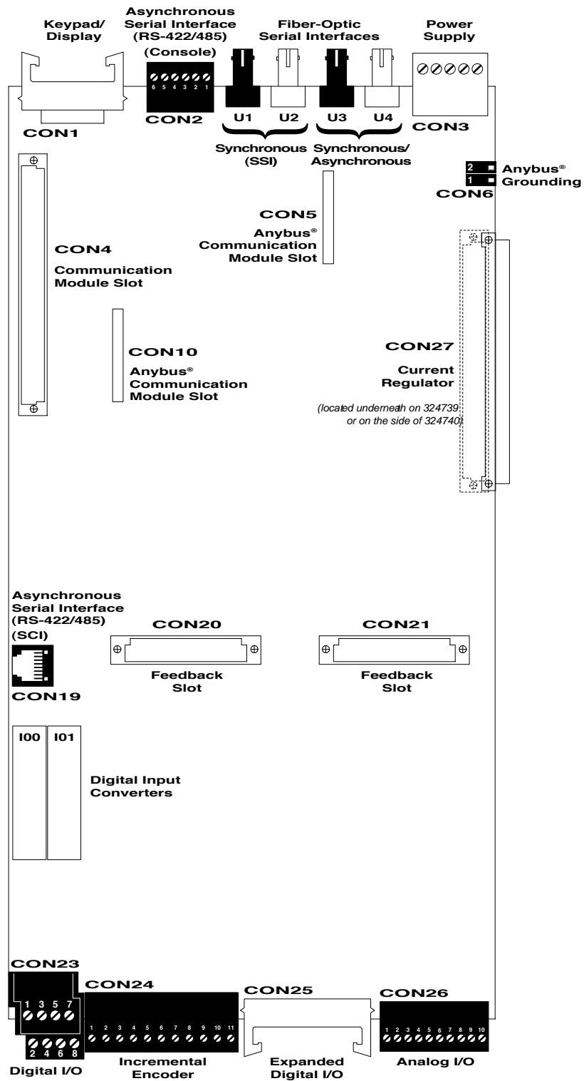
Figure 3-2—270 MHz Expandable Control Module (324739 and 324740)
