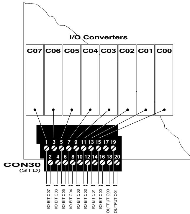
Figure 3-6—On-Board Digital I/O (Standard Control Modules)
