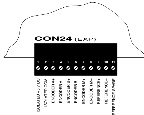
Figure 3-11—On-Board Incremental Encoder Connections
