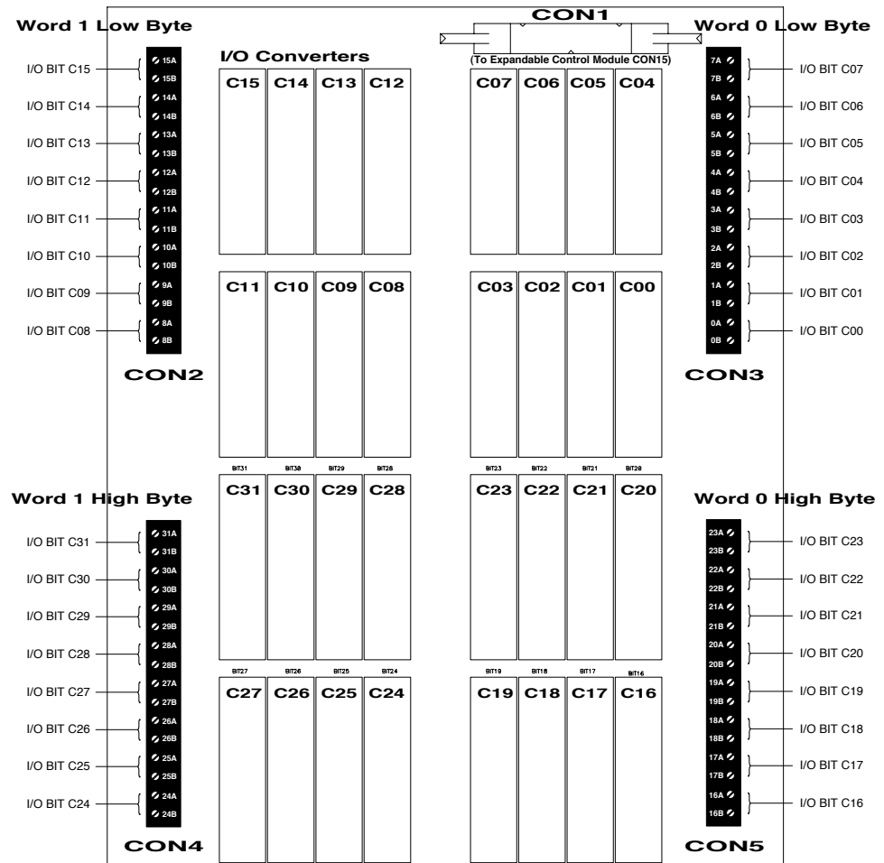
Figure 3-9—32-Bit Fanning Strip Expanded Digital I/O (320146)
