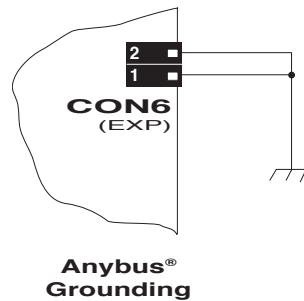
Figure 3-12—Anybus ® Communication Grounding
