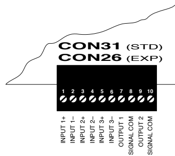
Figure 3-5—Analog I/O Connections
