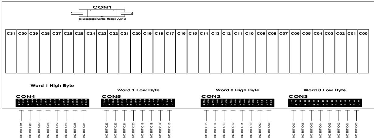
Figure 3-10—32-Bit Fanning Strip Expanded Digital I/O (319437)
