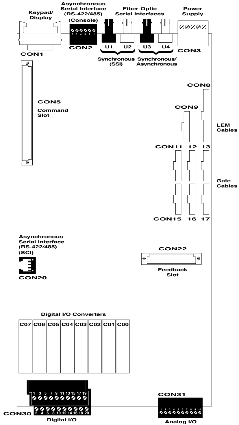
Figure 3-1—270 MHz Standard Control Module (324792, 324793, and 325196)
